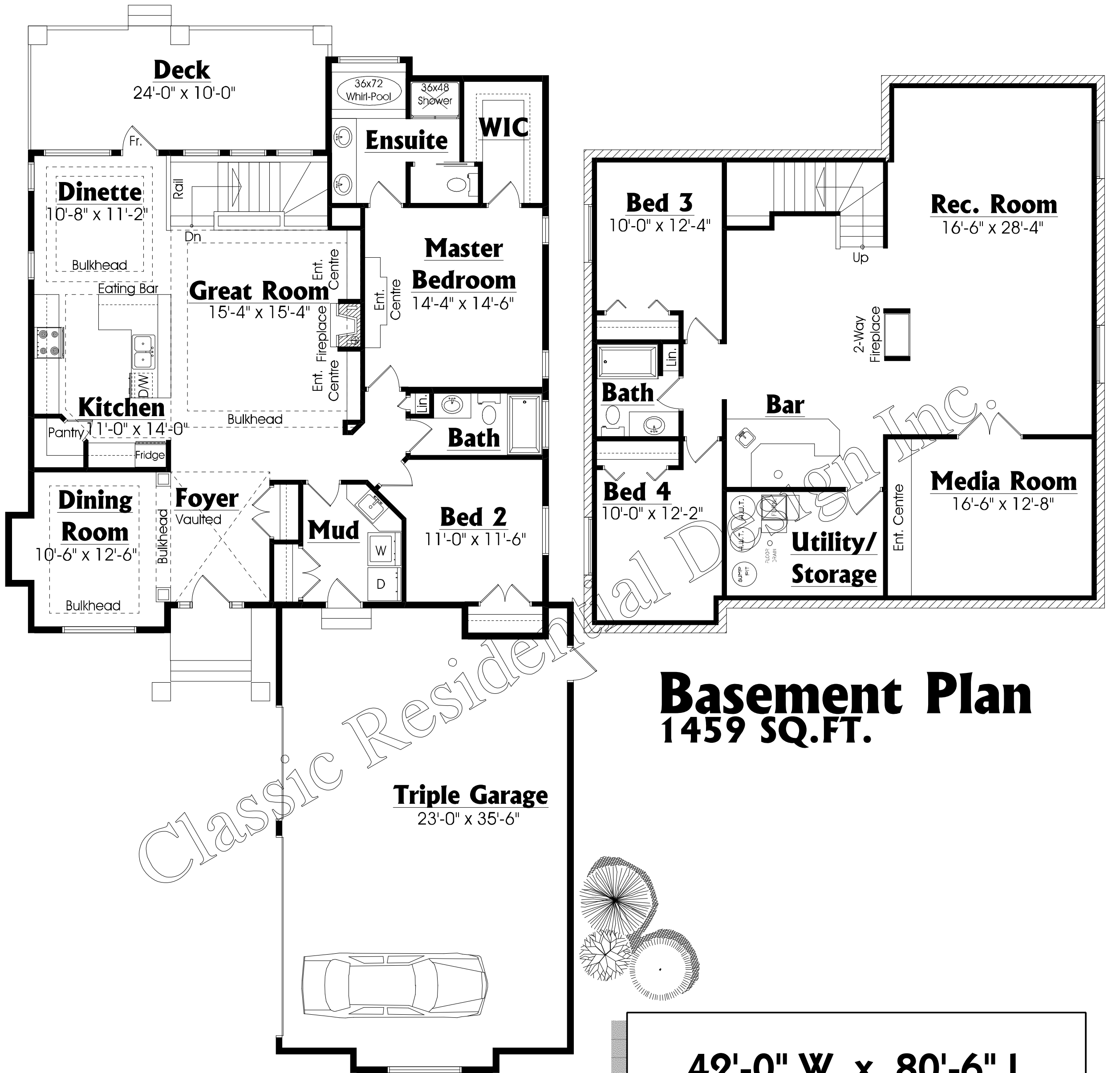
Main Floor Plan 1723 SQ.FT.
