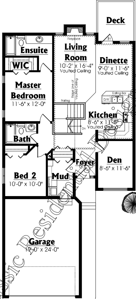
Main Floor Plan 1223 SQ.FT.
