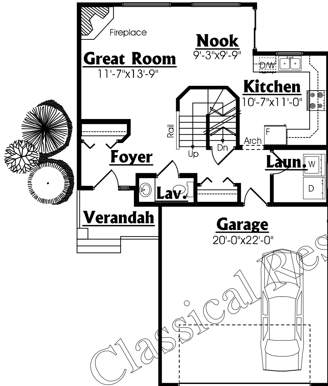
Main Floor Plan 707 SQ.FT.
