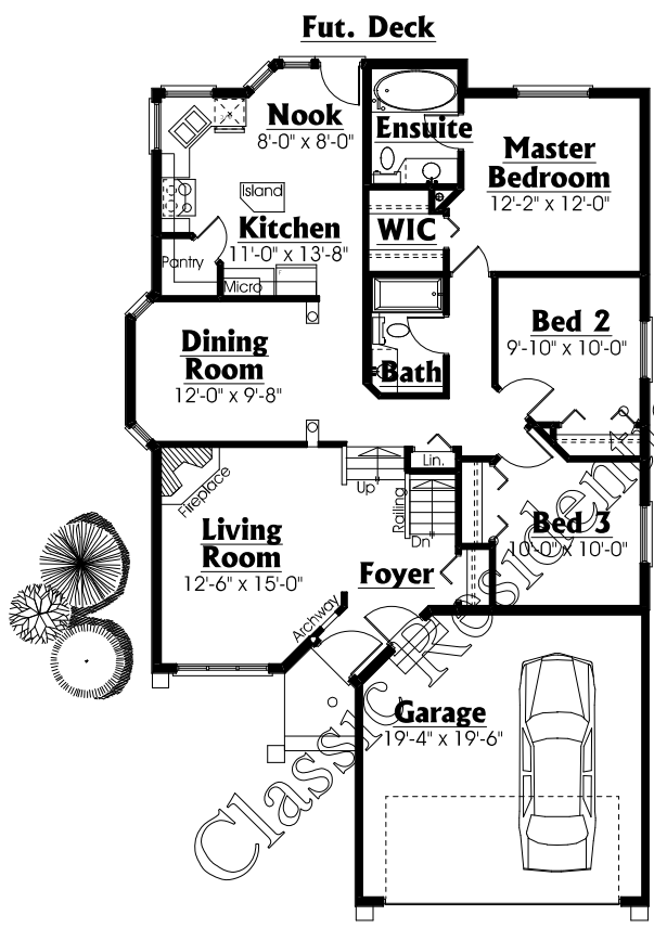
Main Floor Plan 1346 SQ.FT.
