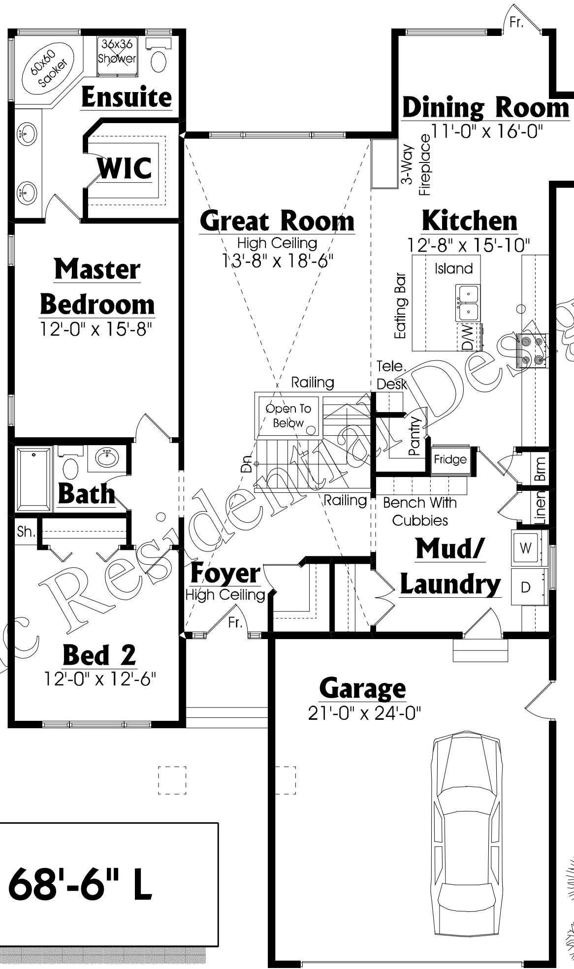
Main Floor Plan 1757 SQ.FT.
