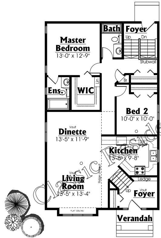
Main Floor Plan 1303 SQ.FT.
