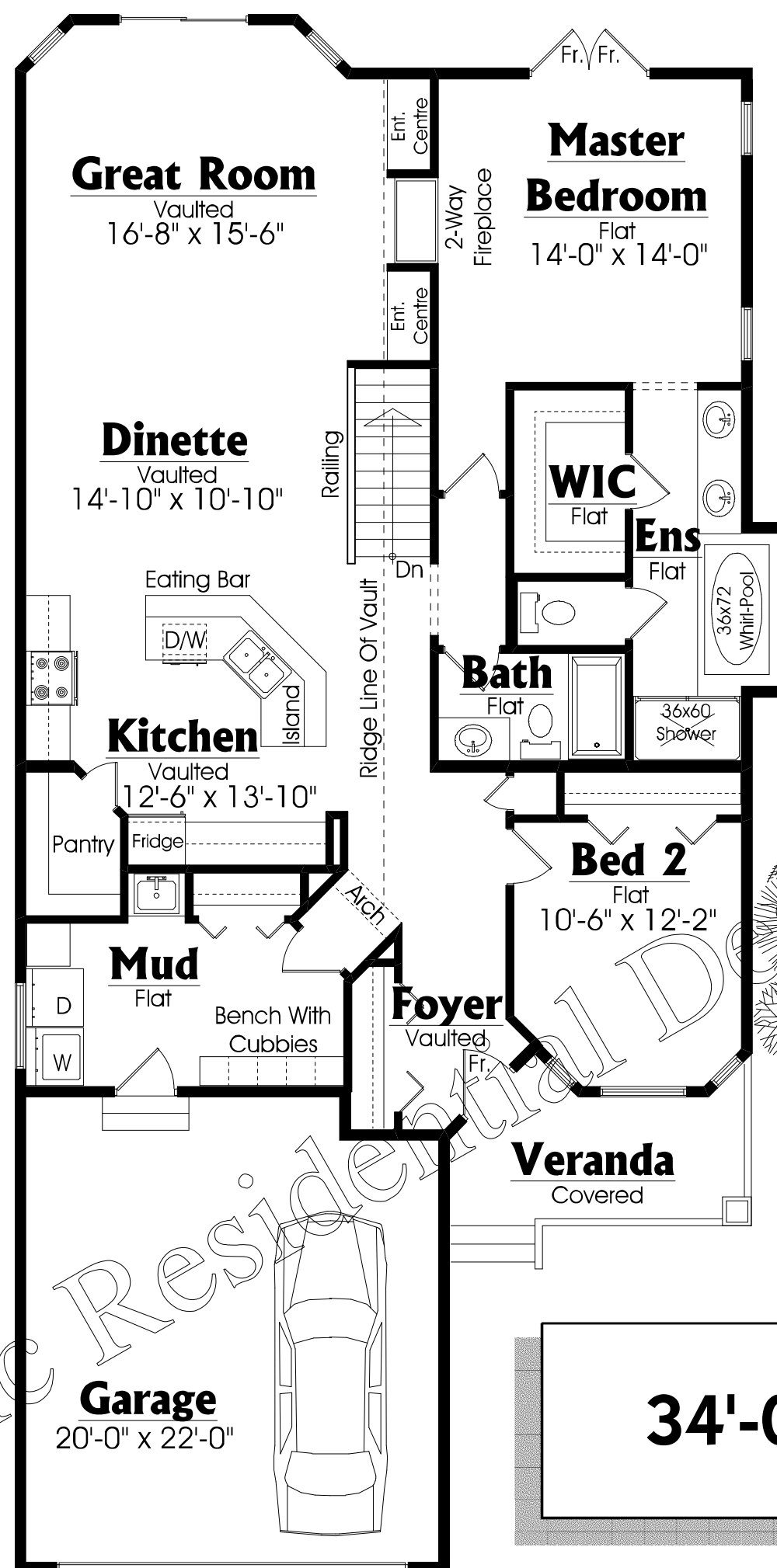
Main Floor Plan 1668 SQ.FT.
