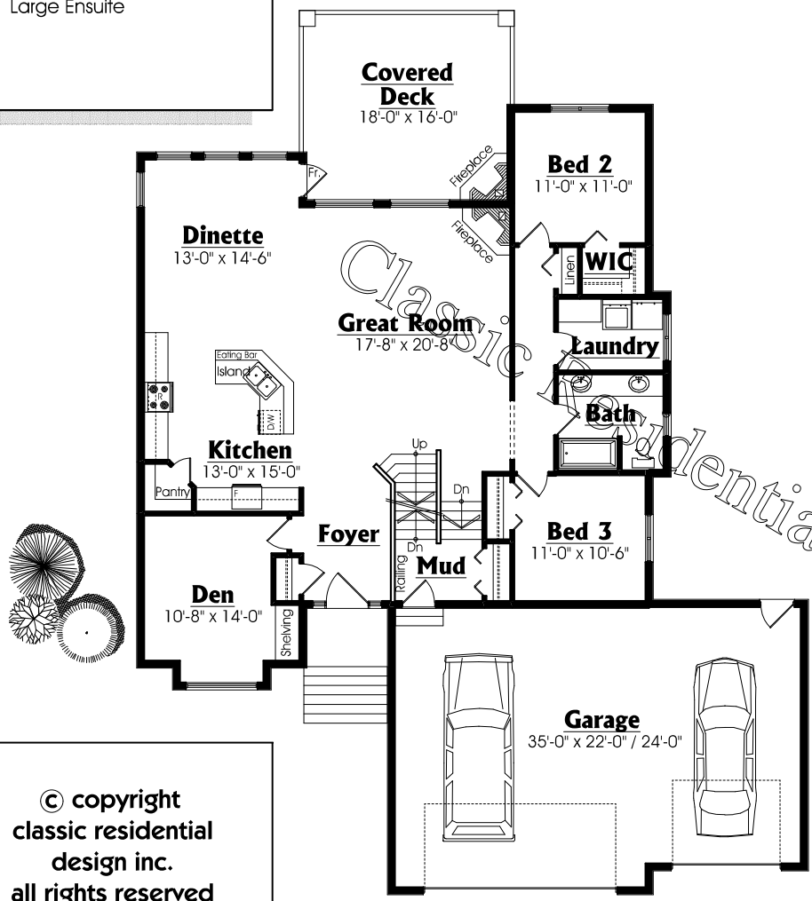
Main Floor Plan 1726 SQ.FT.
