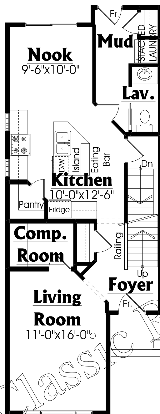
Main Floor Plan 757 SQ.FT.
