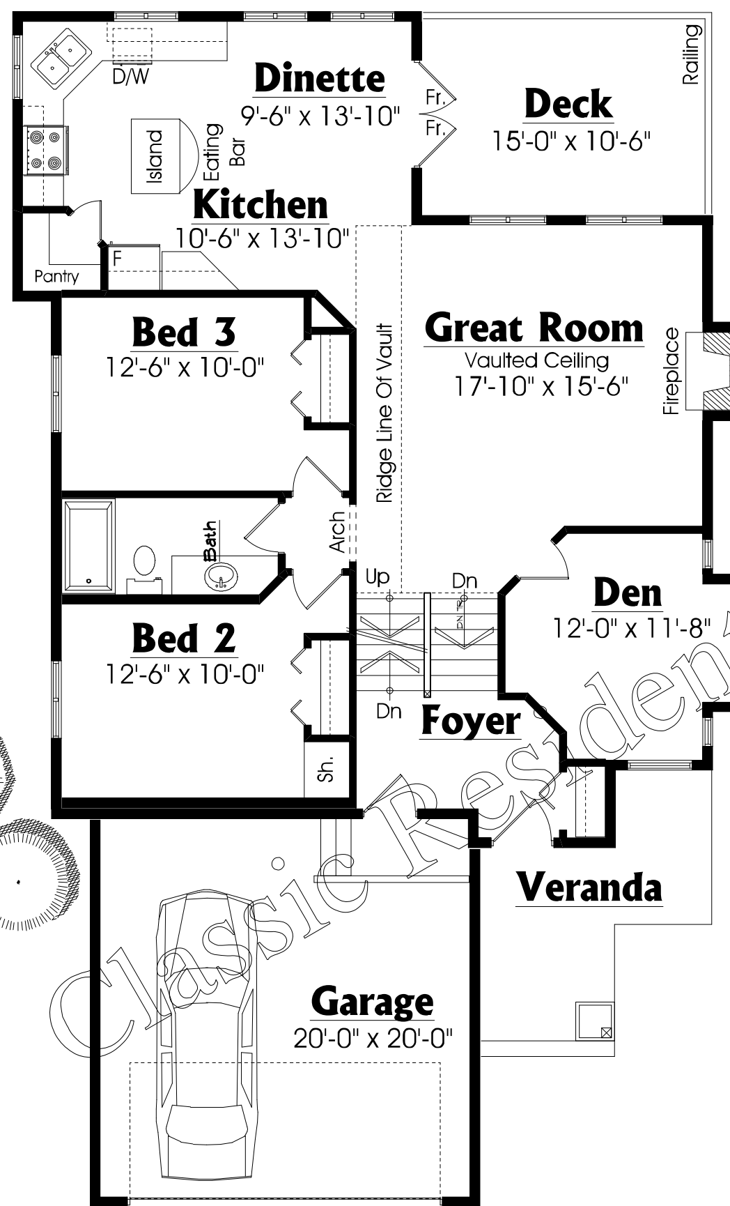
Main Floor Plan 1304 SQ.FT.
