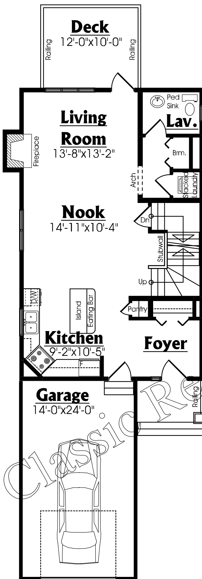
Main Floor Plan 770 SQ.FT.
