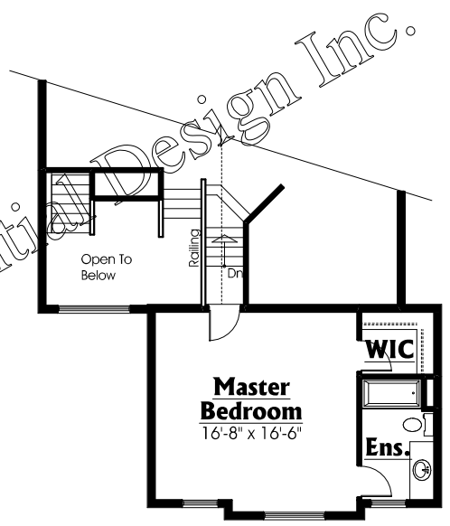
Second Floor Plan 407 SQ.FT.
