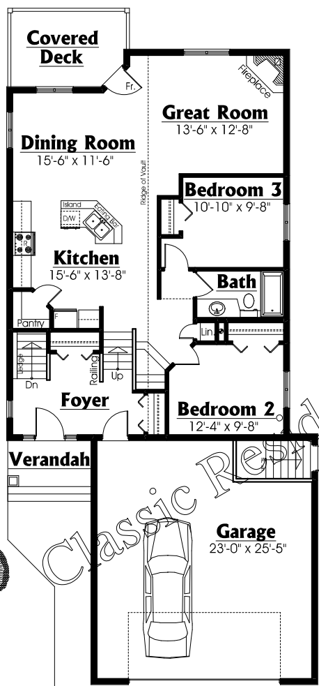
Main Floor Plan 1197 SQ.FT.
