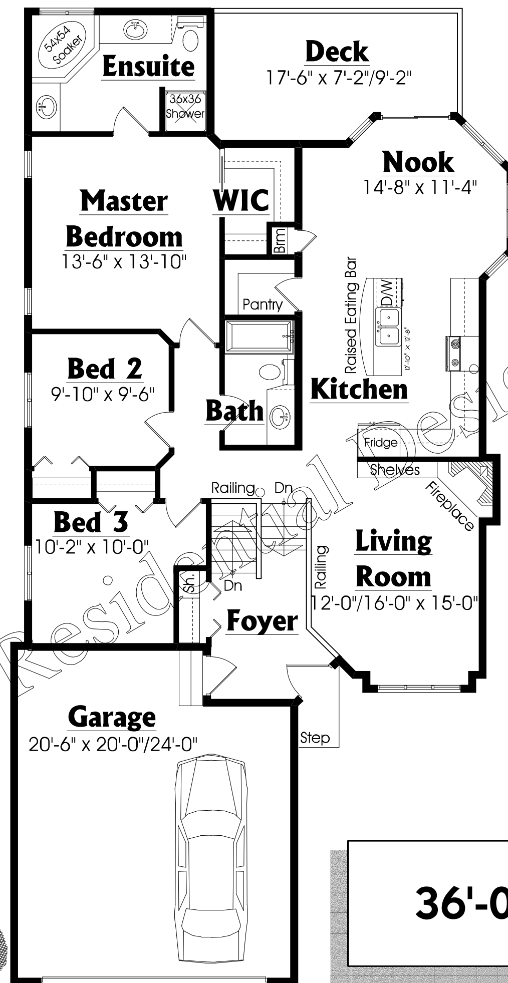
Main Floor Plan 1433 SQ.FT.
