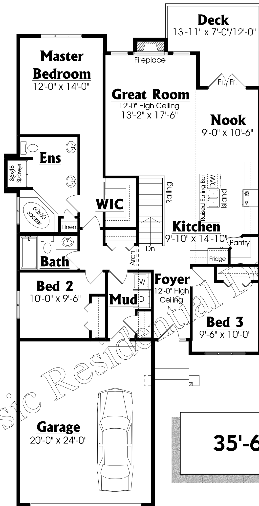
Main Floor Plan 1520 SQ.FT.
