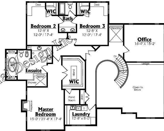
Second Floor Plan 2114 SQ.FT.
